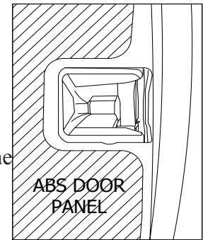
Fig. 2 PASSENGER-SIDE SHOWN
