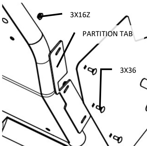
A. With assistance, bolt partition to mounting plate as shown.
